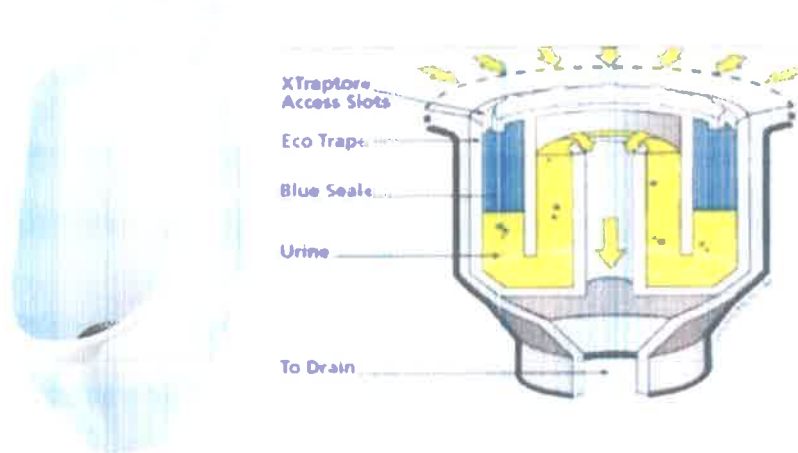
Waterless Urinal
